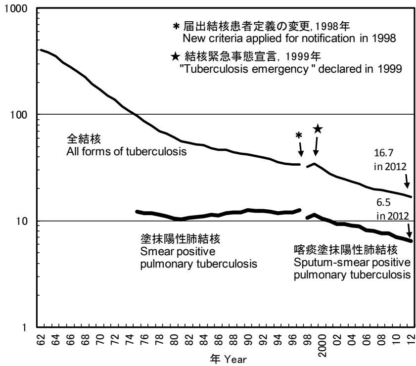
図 1 人口10万対年間新結核患者登録数の年次推移, 1962~2012年 Fig. 1 Annual trend of tuberculosis notification rate (all forms, sputum-smear positive pulmonary tuberculosis) per 100,000 population in Japan, 1962-2012
